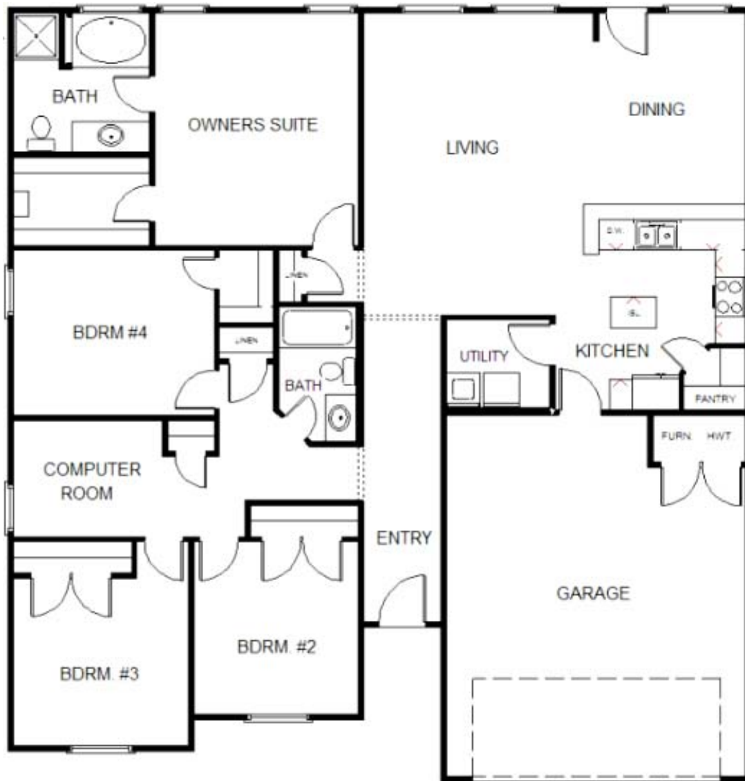
WINDSOR HOMES THE HADLEY 4 BEDROOM PLAN # 1884
